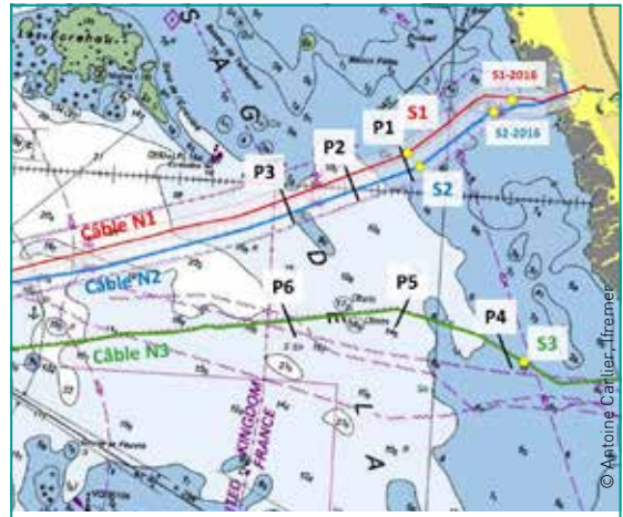
Fig. 9: Positions of the profiles (P1 to P6) and stations (S1 to S3) initially planned for measuring the electromagnetic fields along the Jersey-Cotentin connection comprising the N1, N2 and N3 cables, using the PASSEM tool.
