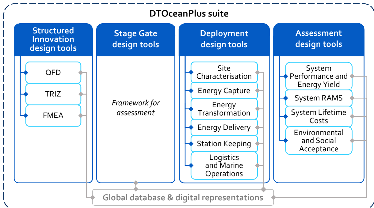
FIGURE o.1 REPRESENTATION OF THE DTOCEANPLUS TOOLS HIERARCHY
