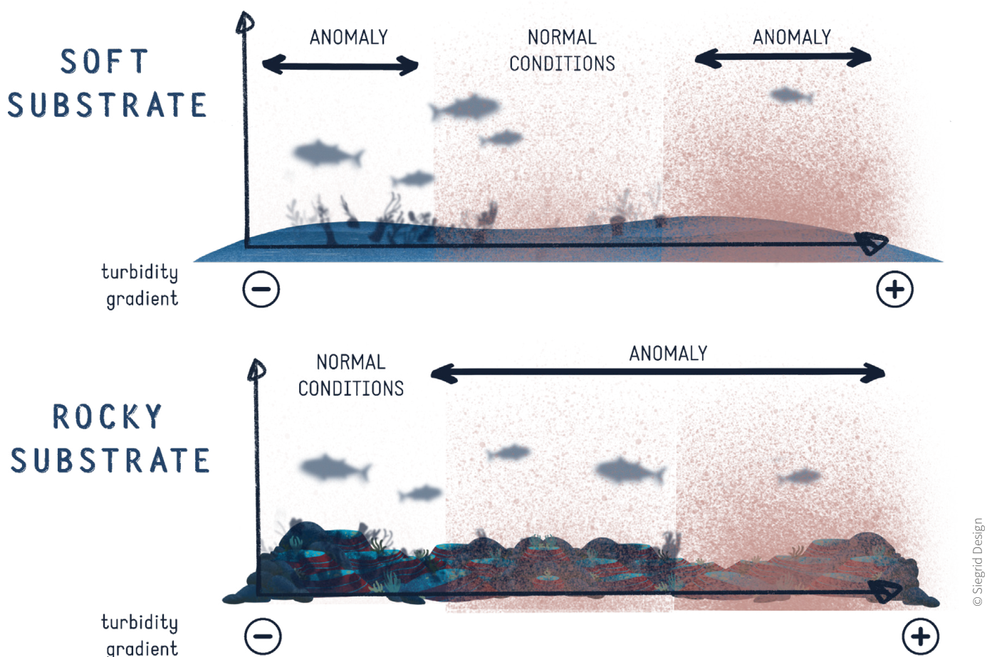
Fig. 1 Concept of a turbidity “anomaly” for two types of substrates: soft and rocky.
