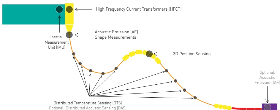
Figure 4: Schematic view of a generic monitoring configuration for dynamic cable
