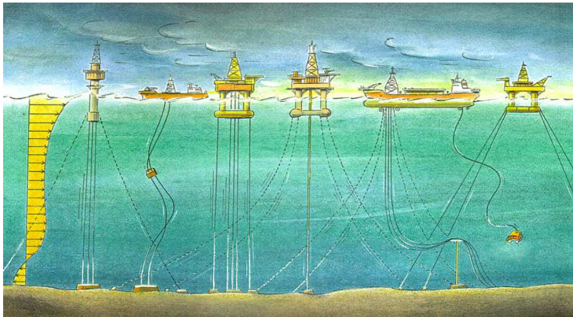
Figure 20: Examples of risers and moorings that can be modelled with Reflex/Mimosa.
