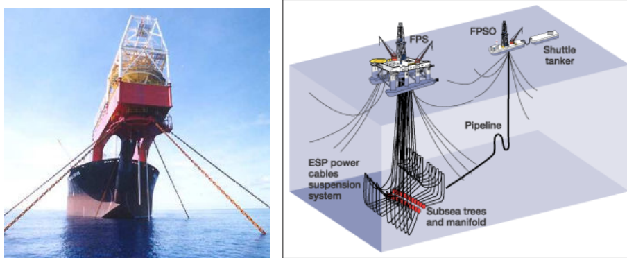
Figure 9: Offshore mooring system examples (left) Buffalo Venture FPSO with single point (taut) mooring and turret system. (right) Schematic of the Liuhua 11-1 semi-submersible platform and shuttle tanker moored with catenary lines
