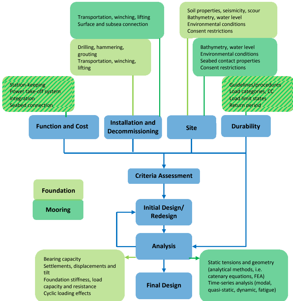
Figure 3: Steps in mooring and foundation design. Considerations specific to moorings (dark green) and foundations (light green) and common requirements (hatched) are shown.
