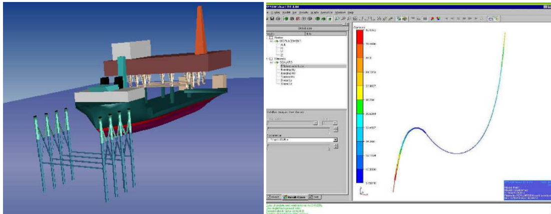
Figure 19: Vessel and structure modelled in Simo ( left ), screenshot showing analysis of flexible object with Reflex ( right )
