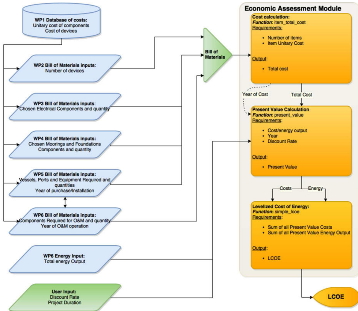
Figure 3.2: Schematic overview of the LCOE calculation in the DTOcean tool
