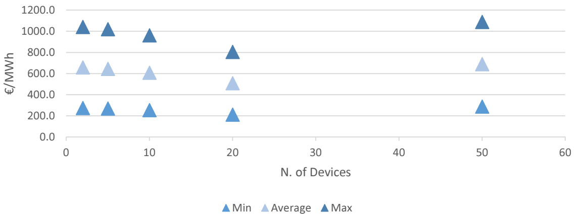
Figure 4.20: LCOE variation
