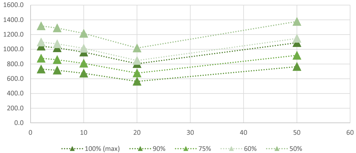
Figure 4.21: LCOE variation for different availability/energy output cases
