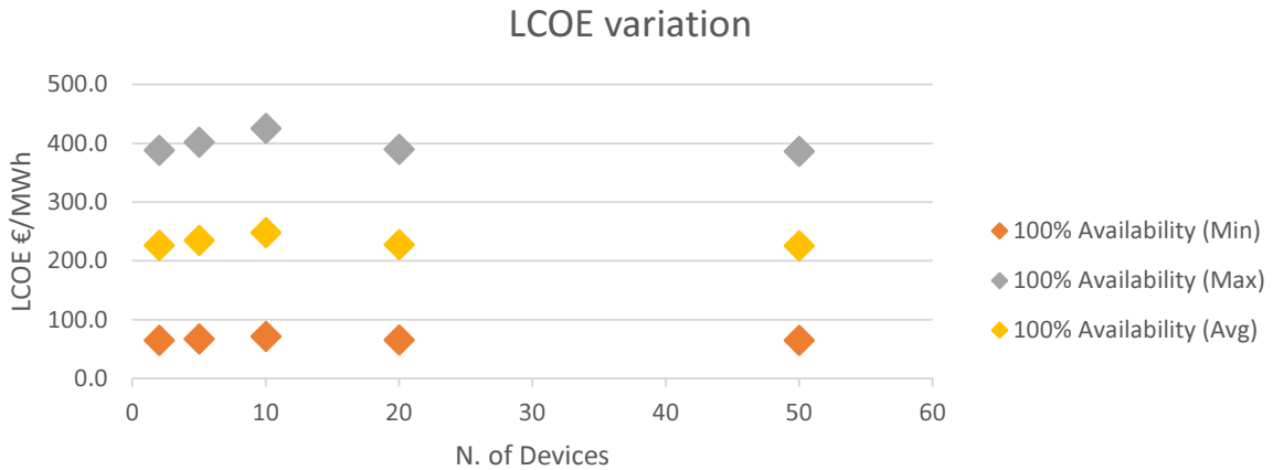
Figure 4.9: LCOE variation
