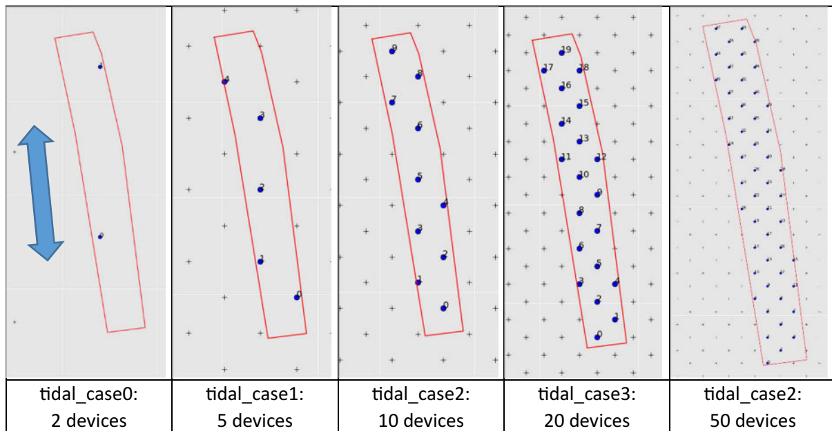
Figure 4.14: Array layout for Scenario 5 The blue arrow indicates flow direction
